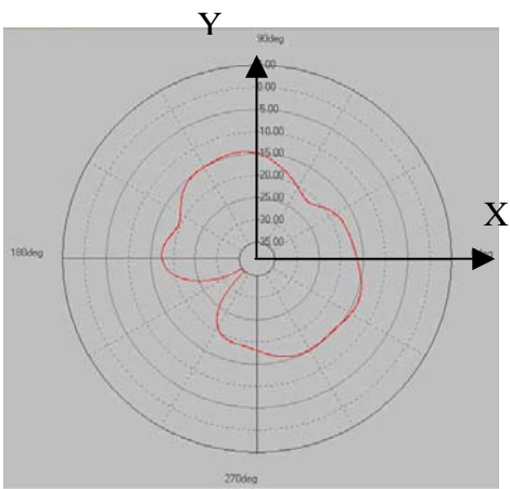
Peak Gain -14.21\text{dBi}
