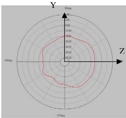
Peak Gain -11.07\text{dBi}
