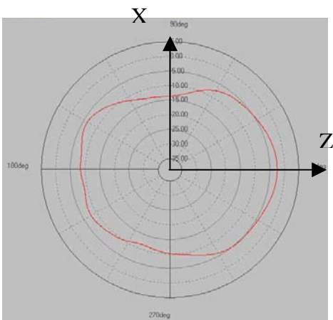
Peak Gain -2.42dBi
