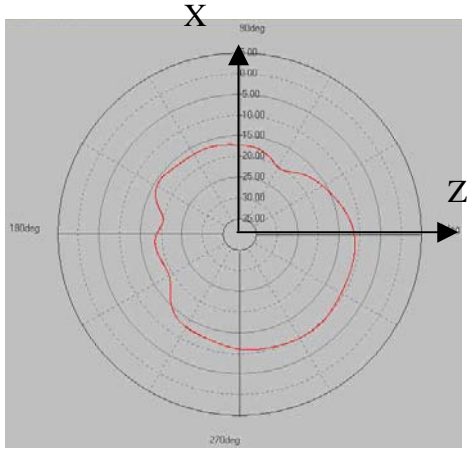
Peak Gain -9.84dBi
