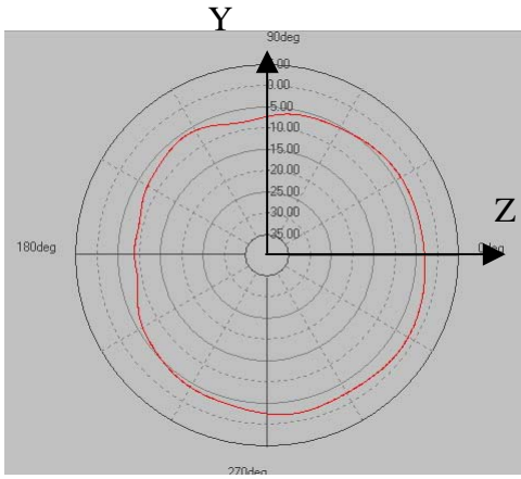
Peak Gain -1.57\text{dBi}
