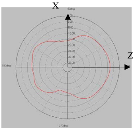
Peak Gain -3.01dBi
