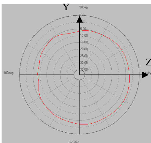
Peak Gain -1.16\text{dBi}
