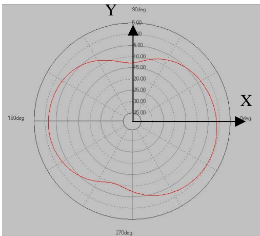
Peak Gain -0.34\text{dBi}
